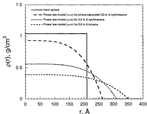
Figure 8. Radial density profile for the power law model and hard sphere model (for comparison).
