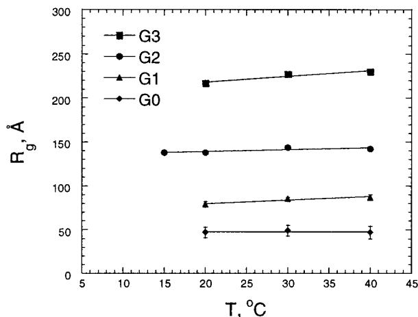
Figure 3. R_g for arborescent graft polymers in d -cyclohexane versus temperature.
