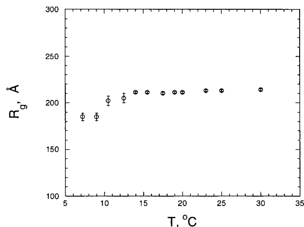
Figure 10. R_g for generation 3 polymer in d -cyclohexane versus temperature showing the collapse of the molecule upon phase separation.
