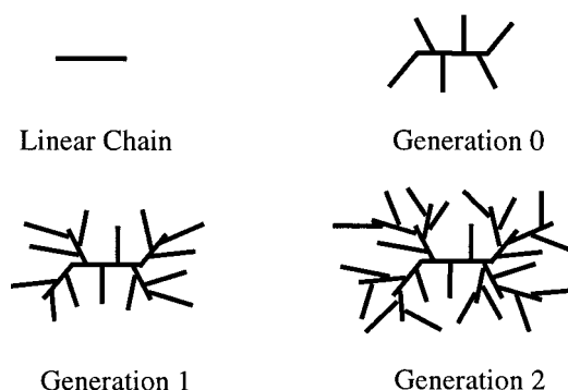
Figure 1. Schematic representation of the growth of arborescent graft polymers by successive cycles of chloromethylation and anionic grafting reactions.
