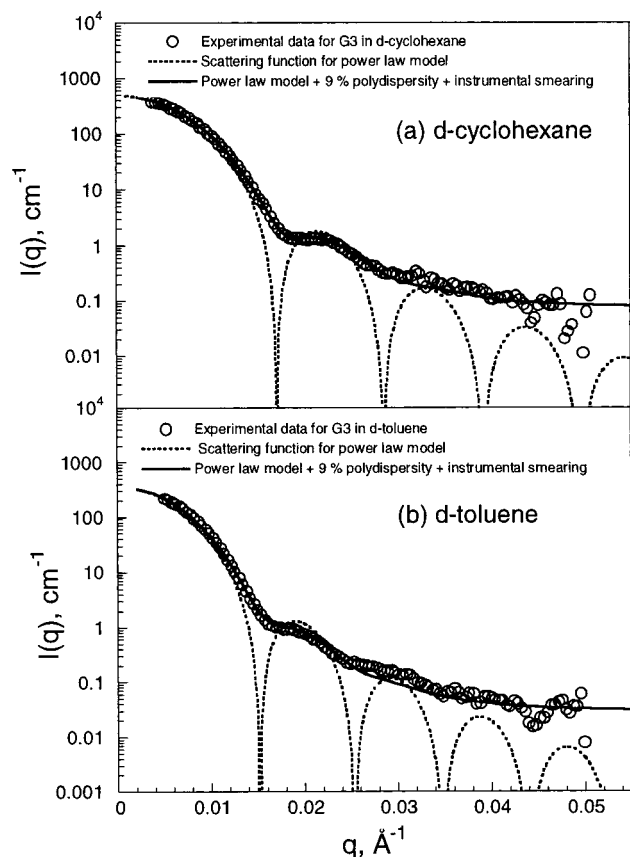
Figure 7. (a) Scattering calculated using the power law model compared experimentally measured scattering for generation 3 polymer in d -cyclohexane. (b) Scattering calculated using the power law model compared with experimentally measured scattering for generation 3 polymer in d -toluene.
