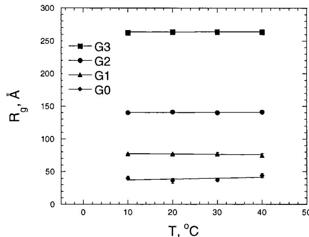
Figure 4. R_g for arborescent graft polymers in d -toluene versus temperature.
